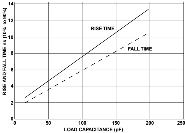
Figure 43. Typical Rise and Fall Times (10% to 90%) vs. Load Capacitance for Driver A at V_{DDEXT} = 2.7\text{ V (MIN)}
