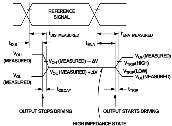
Figure 41. Output Enable/Disable
