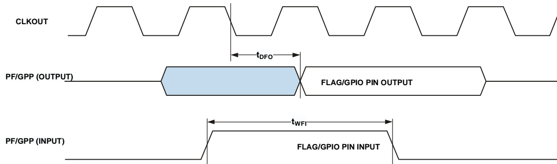
Figure 27. Programmable Flags and GPIO Cycle Timing
