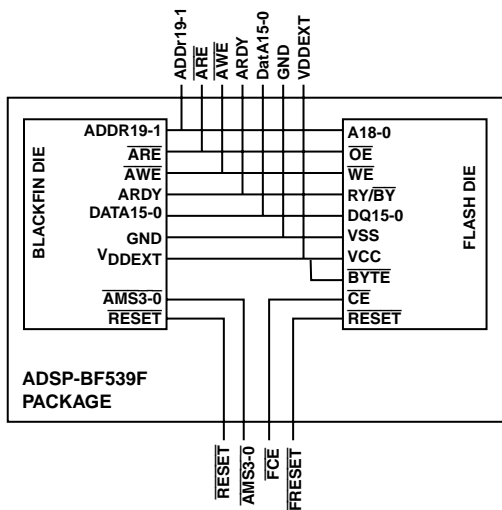
Figure 4. Internal Connection of Flash Memory (ADSP-BF539Fx)
